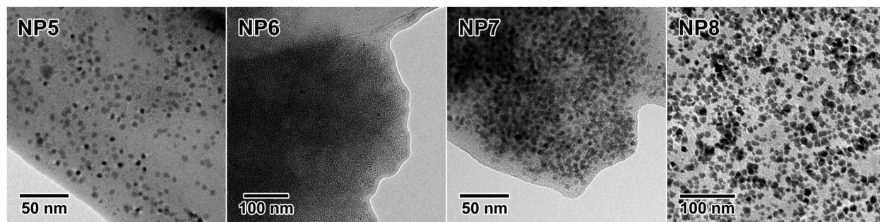
Fig. 2 BF-TEM images of HDA-stabilized colloidal mixed-phase Ni/Ga nanoalloys NP5–7 obtained by co-hydrogenolysis of [\text{Ni}(\text{COD})_2] and \text{GaCp}^* in mesitylene and of NP8 from hydrogenation of [\text{Ni}(\text{GaCp}^*)(\text{PMe}_3)_3] in n -decane.
