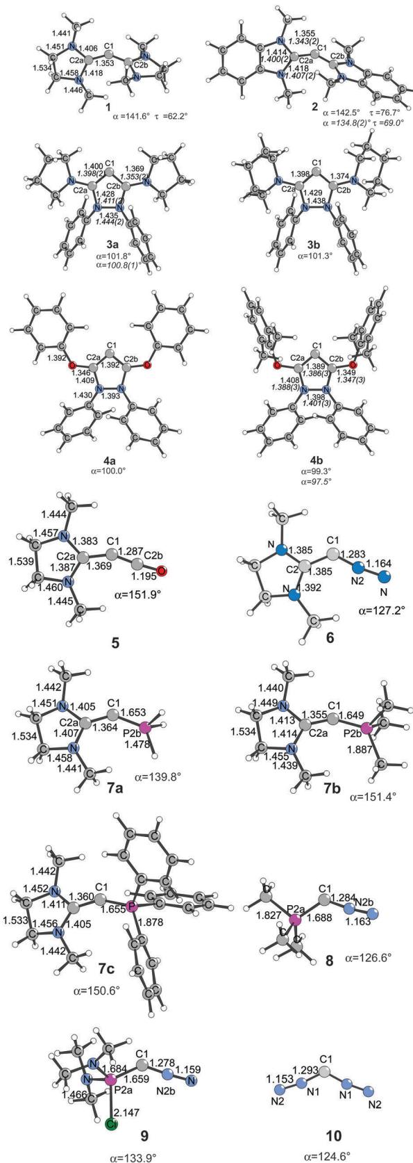
Fig. 6 Calculated (BP86/SVP) geometries of some carbones \text{CL}_1\text{L}_2 . 32 Bond lengths are given in Å, angles in degree. Experimental data are given in italics . 26,34 The figure has been adapted from ref. 32.
