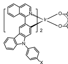
205: X = H
