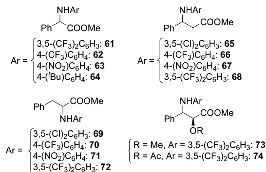
Chart 4 α- and β-amino esters obtained by Ru(TPP)CO-catalysed amination of carboxylic esters.
