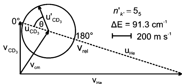
Fig. 2 Newton diagram for inelastic scattering of \text{CD}_3 with helium. The displayed Newton sphere corresponds to the n_k = 1_1 \rightarrow n'_{k'} = 5_5 transition, for which \Delta E = 91.3 \text{ cm}^{-1} .
