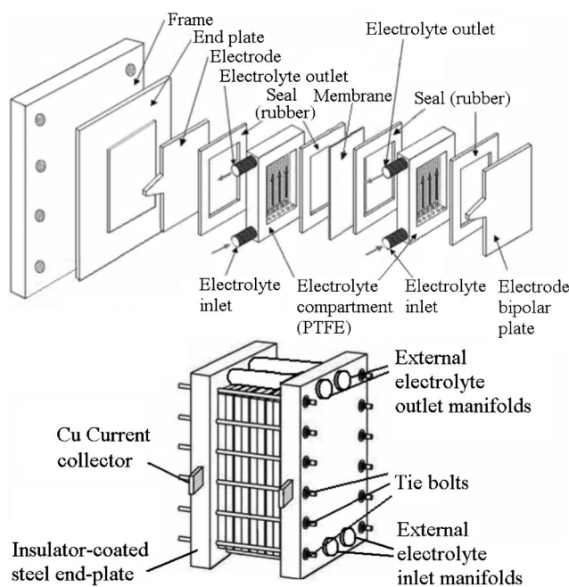
Fig. 7 Components of a flow battery and a cell stack. 200,276,277
