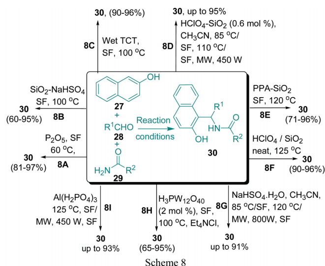
Scheme 8
