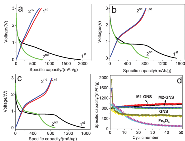
Fig. 9 The initial two charge/discharge curves of (a) original GNS, (b) M1-GNS and (c) M2-GNS, and (d) cycling performance of M1-GNS, M2-GNS, GNS, and \text{Fe}_3\text{O}_4 nanoparticles at the current density of 50\text{ mA g}^{-1} .
