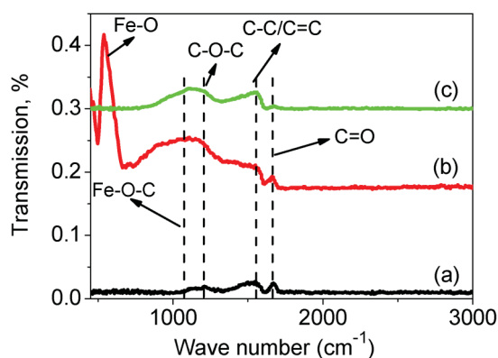
Fig. 8 FTIR transmittance spectra of (a) GNS, (b) M1-GNS and (c) residual graphene sheets from M1-GNS after removing \text{Fe}_3\text{O}_4 nanoparticles.
