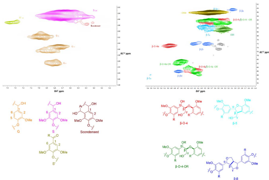
Fig. 6 2D-HSQC NMR of organosolv-extracted birch-wood lignin showing the lignin aromatic subunit region (left) and linking motif region (right) for run B (120 °C, 4 g s solvent min -1 ), done in acetone d 6 .
