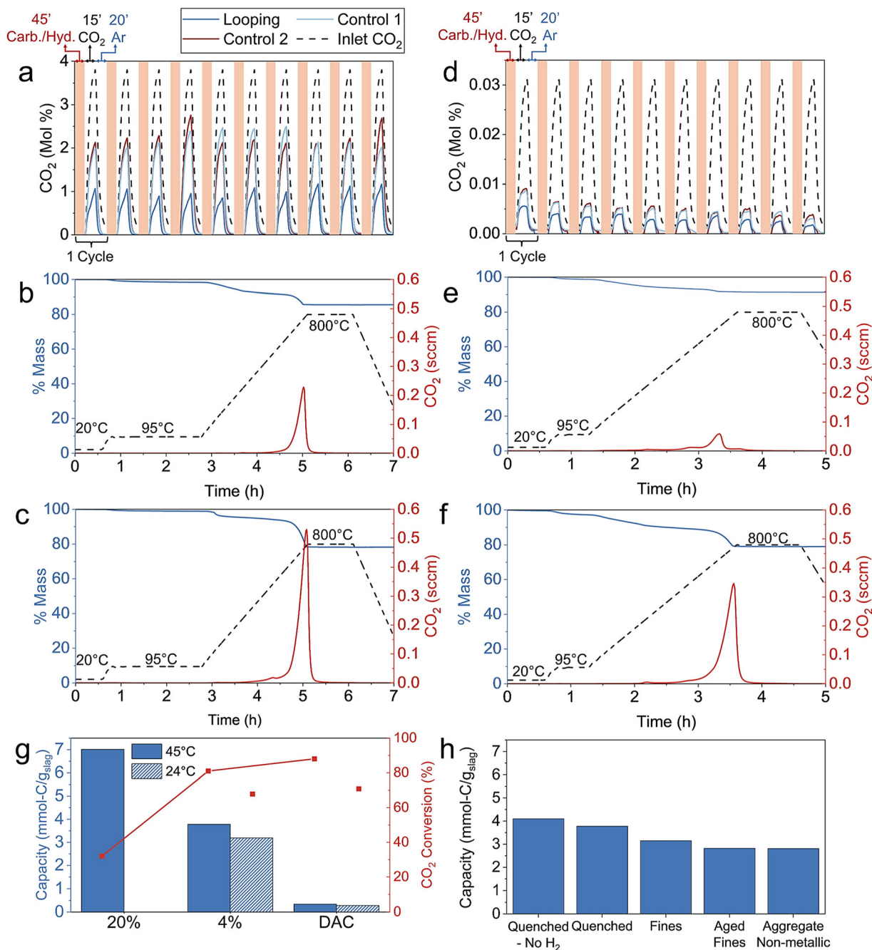
Fig. 5 (a) Ten \text{Na}_2\text{CO}_3 looping and control cycles of point-source \text{CO}_2 capture with quenched BOF slag. 0.5 g of steel slag per cycle with 90 sccm 4% \text{CO}_2 /Ar. (b) Thermogravimetric analysis (TGA) and \text{CO}_2 evolution of carbonate-rich product after 10 cycles from a control method with steel slag and water mixture capturing 4% \text{CO}_2 . (c) TGA and \text{CO}_2 evolution of carbonate-rich product after 10 cycles from \text{Na}_2\text{CO}_3 looping capturing 4% \text{CO}_2 , showing 1.9 times higher \text{CO}_2 mineralization than the control in (b). (d) Ten \text{Na}_2\text{CO}_3 looping and control cycles of air \text{CO}_2 capture with quenched BOF slag. 0.05 g of steel slag per cycle with 90 sccm of 343 ppm \text{CO}_2 /Air. (e) TGA and \text{CO}_2 evolution of carbonate-rich product after 10 cycles from a control method with steel slag and water mixture capturing 343 ppm \text{CO}_2 . (f) TGA and \text{CO}_2 evolution of carbonate-rich product after 10 cycles from air \text{CO}_2 \text{Na}_2\text{CO}_3 looping, showing 4.3 times higher \text{CO}_2 mineralization than the control (e). (g) Comparison of \text{CO}_2 capture capacity and \text{CO}_2 conversion by quenched slag over 5 cycles for 20% \text{CO}_2 , 4% \text{CO}_2 , and 343 ppm \text{CO}_2 (air) at 45 °C and room temperature (24 °C). (h) \text{CO}_2 capture capacity of different BOF slags over 5 cycles for 4% \text{CO}_2 . Quenched - No \text{H}_2 is quenched slag that did not react with steam for \text{H}_2 production prior to \text{Na}_2\text{CO}_3 looping. All cycles were conducted at 45 °C, unless noted otherwise.
