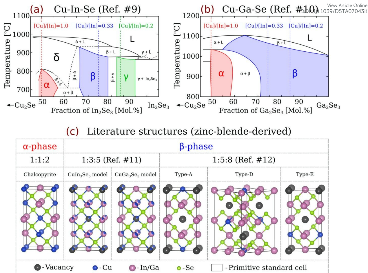
Figure 1. Experimental phase diagram of the pseudo-binary (a) \text{Cu}_2\text{Se}-\text{In}_2\text{Se}_3 system adapted from Ref. #9 and (b) \text{Cu}_2\text{Se}-\text{Ga}_2\text{Se}_3 system adapted from Ref. #10. (c) The most important crystal structures reported for the \alpha - and \beta -phases. The 1:3:5 ODC structural models were resolved using the neutron and X-ray diffraction experiments in Ref. #11. The 1:5:8 ODC structural models were proposed in Ref. #12. A more extensive list of literature structures is given in Table S1.
