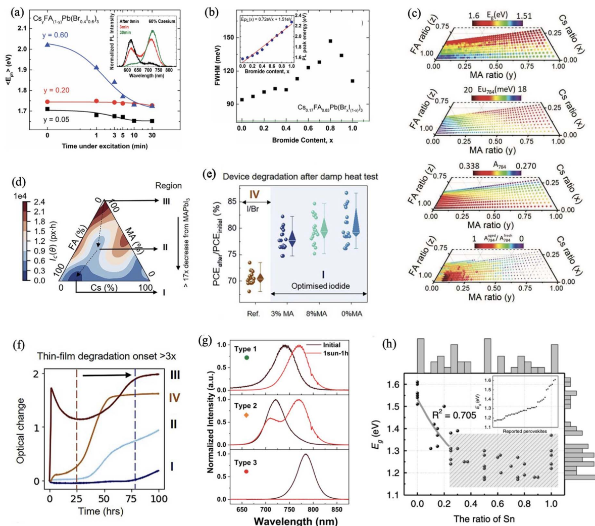
Fig. 1 (a) Changes in average PL emission photon energy ( E_{ph} ) of \text{Cs}_y\text{FA}_{(1-y)}\text{Pb}(\text{Br}_{0.4}\text{I}_{0.6})_3 films at y = 0.05 , y = 0.20 and y = 0.60 . (b) FWHM of the PL emission spectra of \text{Cs}_{0.17}\text{FA}_{0.83}\text{Pb}(\text{Br}_{x(1-x)})_3 films as a function of \text{Br}^- content x . Inset shows the correlation between PL peak energy and \text{Br}^- content with fitting function. Reproduced from ref. 62 with permission from The Royal Society of Chemistry, copyright 2017. (c) Ranges of bandgap ( E_g ), Urbach energy ( E_{u784} ), absorbance ( A ) and aged to fresh absorbance ratio ( A_{\text{aged784}}/A_{\text{fresh784}} ) of \text{Cs}_x\text{MA}_y\text{FA}_z\text{PbI}_3 alloys at 520 nm locations. Reproduced from ref. 63 with permission from Wiley-VCH GmbH, copyright 2023. (d) Non-linear instability landscape ( I_c(\theta) ) within the \text{Cs}_x\text{MA}_y\text{FA}_{1-x-y}\text{PbI}_3 compositional space with stability in the order of Region I > Region II > Region III. (e) Comparison of percentage ratios of PCEs after damp heat degradation tests between Region IV I/Br-based PSCs and Region I I-based PSCs. (f) Optical changes as a function of degradation time showing Region I as the most stable region. Reproduced from ref. 34 with permission from Elsevier Inc., copyright 2021. (g) Normalized PL peaks of the photodegradation of materials showing three different degradation pathways denoted as Type 1, Type 2 and Type 3. Reproduced from ref. 21 with permission from Elsevier Inc., copyright 2023. (h) Fitted plot of bandgap ( E_g ) as a function of Sn : Pb ratio for 43 reported perovskites and histograms indicating corresponding distributions with respect to Sn : Pb ratio and bandgap. Inset is the bandgap values of the perovskites in ascending order. Reproduced from ref. 77 with permission from Springer Nature Ltd, copyright 2022.
