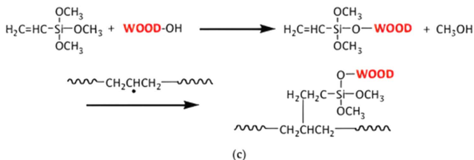
Fig. 7 Possible reactions of coupling agents: (a) MAPE, (b) Si69 and (c) VTMS with wood fibres. Reprinted with permission. 76 Copyright 2018, MDPI.
