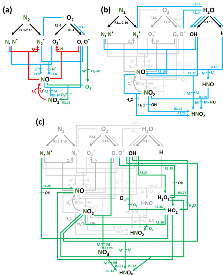
Fig. 2 Reaction diagrams of the N 2 oxidation processes in (a) N 2 : O 2 (air), (b) N 2 + H 2 O and N 2 + O 2 (air) + H 2 O feedstocks, where (c) highlights the chemistry in the plasma/liquid interface. Black, blue, red, and green arrows indicate electron impact reactions, forward reactions, reverse reactions at high temperature, and reactions pronounced at low temperature, respectively.
