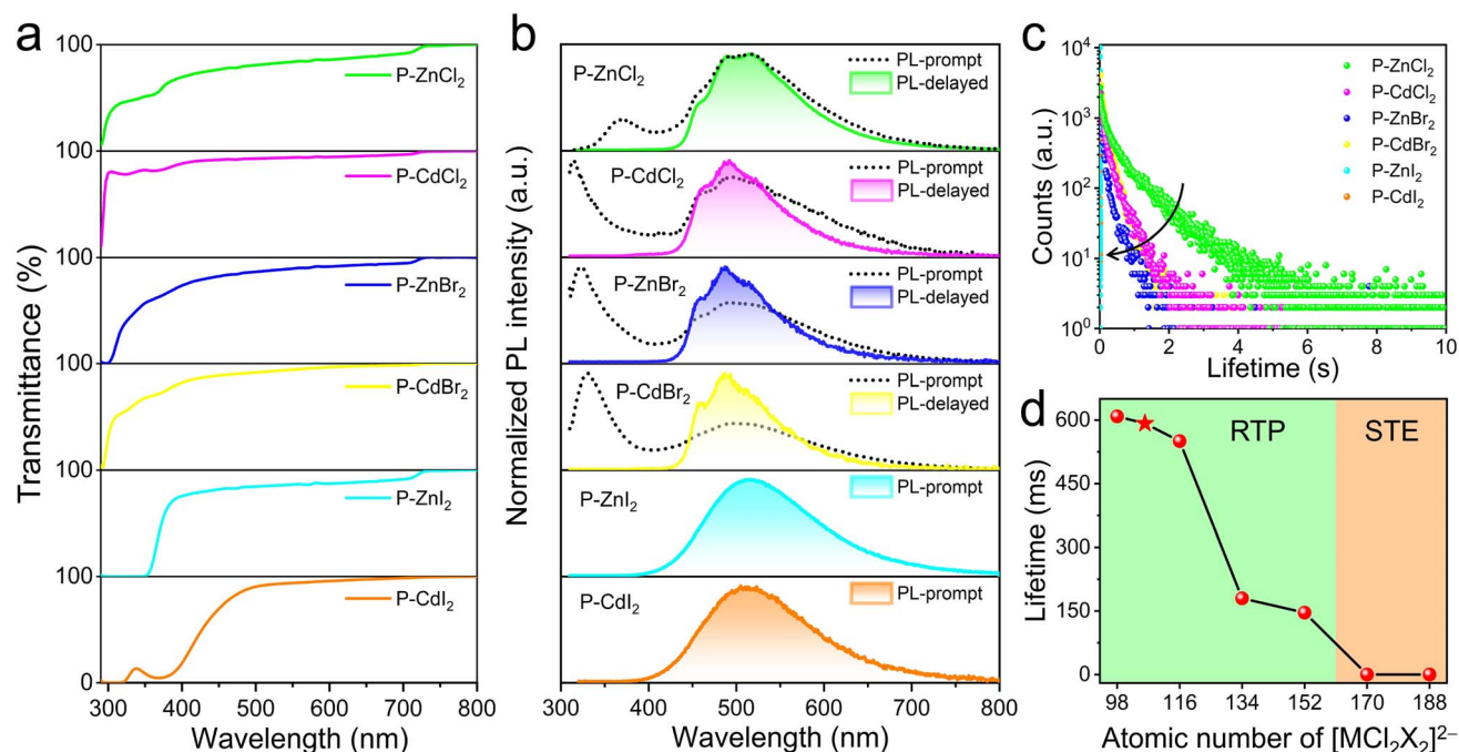
Fig. 3 (a) Transmittance spectra of (\text{BuTPP})_2\text{MCl}_2\text{X}_2 glasses. (b) The prompt and delayed PL spectra of (\text{BuTPP})_2\text{MCl}_2\text{X}_2 glasses. (c) Time-resolved phosphorescence decay curves of (\text{BuTPP})_2\text{MCl}_2\text{X}_2 glasses. (d) The phosphorescence lifetimes of (\text{BuTPP})_2\text{MCl}_2\text{X}_2 glasses as a function of atomic number of [\text{MCl}_2\text{X}_2]^{2-} in (\text{BuTPP})_2\text{MCl}_2\text{X}_2 glasses.
