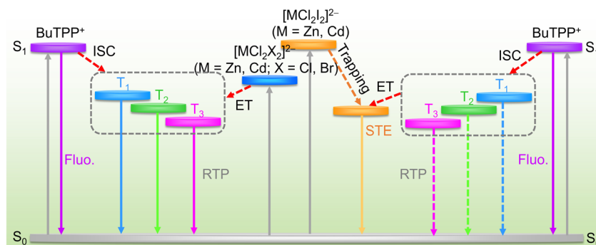
Fig. 4 Schematic illustrations of the excited states alignments, energy transfer and relaxation paths of excited states in (\text{BuTPP})_2\text{MCl}_2\text{X}_2 glasses.
