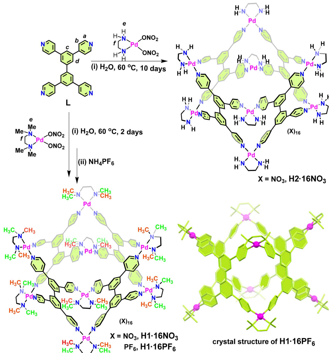
Fig. 2 Synthesis of the polycationic molecular cuboids [Pd 8 (tmeda) 8 (L) 4 ](X) 16 (X = NO 3 : H 1 ·16NO 3 ; X = PF 6 : H 1 ·16PF 6 ), and [Pd 8 (en) 8 (L) 4 ](NO 3 ) 16 , H 2 ·16NO 3 . Crystal structure of H 1 ·16PF 6 showing the [Pd 8 (tmeda) 8 (L) 4 ] 16+ architecture (counter anions and H atoms are not shown for clarity).
