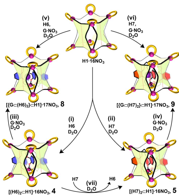
Fig. 5 Designer coordination cage (\text{H1})^{16+} as super-host \text{H}_{\text{out}} for encapsulation of (i) and (ii) two units of typical crown ethers ( \text{H6}/\text{H7} ) as \text{H}_{\text{in}} to form [(\text{H}_{\text{in}})_2 \subset (\text{H}_{\text{out}})] . (iii) and (iv) Addition of \text{Cs}^+ as G after accommodation of the two units of crown ether to form [(\text{G}) \subset (\text{H}_{\text{in}})_2] \subset (\text{H}_{\text{out}}) . (v) and (vi) Combination of one equivalent of \text{Cs}^+ ions and two equivalents of typical crown ethers in a single pot to form [(\text{G}) \subset (\text{H}_{\text{in}})_2] \subset (\text{H}_{\text{out}}) . (vii) Encapsulation of one crown ether over another in a selective manner, showing the preference for H7 over H6 (the behaviour of H8 is found to be comparable with that of H7 ).
