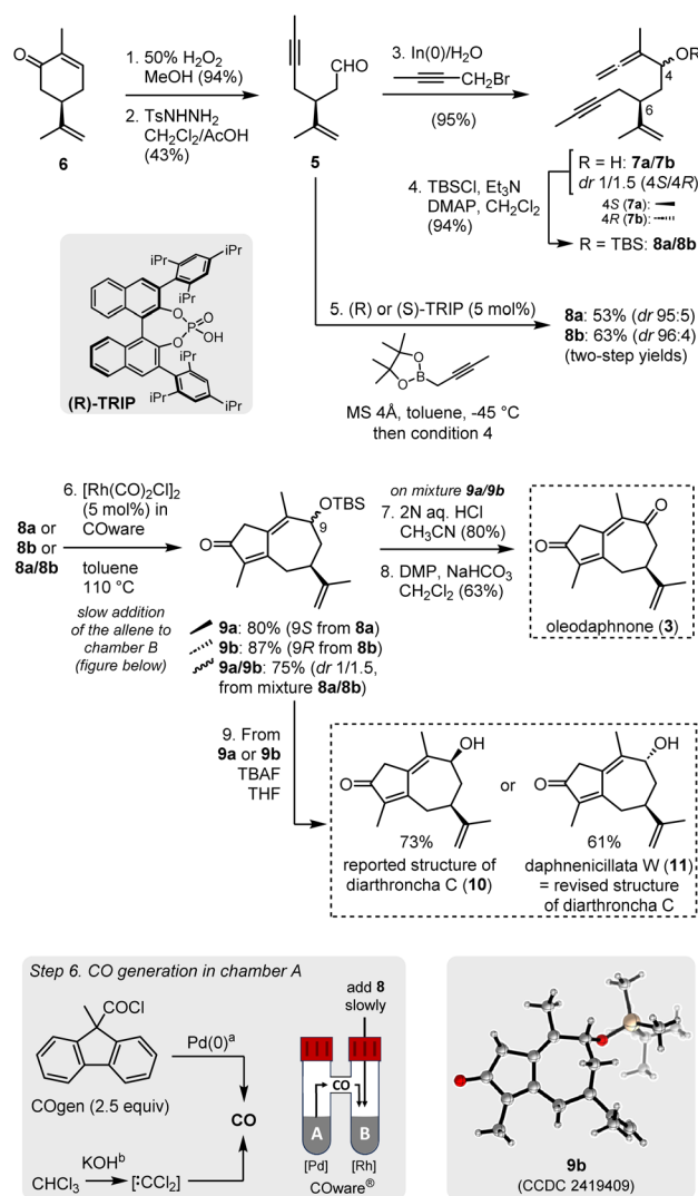
Scheme 2 Total synthesis of oleodaphnone ( 3 ), diarthroncha C ( 10 , structure as reported in the literature), and daphnencillata W ( 11 ), through an APKR performed in COWare®. Notes: (a) COgen (2.5 equiv.), PdCl 2 (cod) (10 mol%), [( t -Bu) 3 PH]BF 4 (10 mol%), MeN(Cy) 2 (4.0 equiv.), toluene (0.02 M); 36 (b) KOH (30 equiv.), CHCl 3 (10 equiv.), toluene (0.05 M). 37 Note: ORTEP structure of 9b at 50% probability level (CCDC number: 2419409). †1
