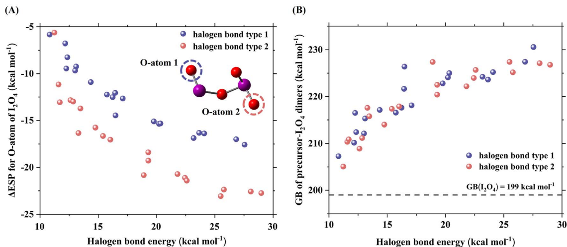
Fig. 3 Change in electrostatic potential ( \Delta\text{ESP} ) values (kcal mol ^{-1} ) for the O atom as a basic site of \text{I}_2\text{O}_4 (A) and the gas basicity (GB) (kcal mol ^{-1} ) of precursor- \text{I}_2\text{O}_4 dimers (B) as a function of the halogen bond energy (kcal mol ^{-1} ). The purple and red spheres represent two different types of XBs. O-atom 1 is the basic site of \text{I}_2\text{O}_4 when it forms XB type 1 with precursors. O-atom 2 is the basic site of \text{I}_2\text{O}_4 when it forms XB type 2 with precursors.
