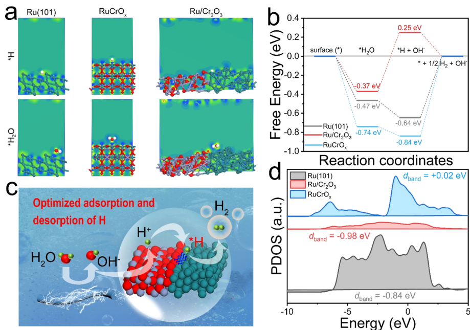
Fig. 5 (a) The charge differential density maps of the adsorption of \text{H}^* and \text{H}_2\text{O}^* on Ru(101), RuCrO x and Ru/Cr 2 O 3 models, where blue and yellow represent electron density decrease and increase, respectively. The green, cyan and red spheres represent Ru, Cr and O atoms, respectively. (b) Calculated adsorption energies of \text{H}_2\text{O}^* and \text{H}^* on the surface for Ru(101), RuCrO x and Ru/Cr 2 O 3 models. (c) Schematic illustration of the proposed HER catalytic mechanism on Ru/Cr 2 O 3 HNFs. (d) The PDOS of Ru atoms for Ru(101), RuCrO x and Ru/Cr 2 O 3 models.
