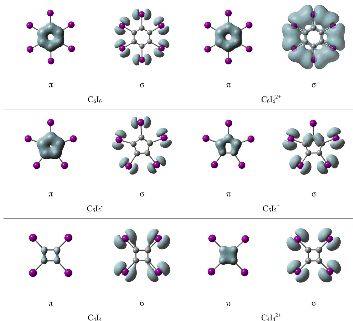
Fig. 5 Isosurface of the EDDB _{\pi} function calculated for \pi -electrons (isovalued at 0.01 a.u.) and for \sigma -electrons (isovalued at 0.001 a.u.).
