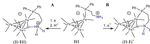
Scheme 2 Presentation of possible H-bond stabilization that enables observation of (\text{H}-1\text{H})^{0/-} or (\text{H}-1\text{a})^{2-} , couple at -1.63 V. (A) Proton source is from bulk solution; (B) proton source for hydride formation is the amine SCS group.
