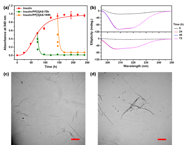
Fig. 5 (a) Disintegration of preformed insulin fibrils by PP[3]AS ( 344 \mu\text{M} ), where the disintegrator was added to aggregating solution of 172 \mu\text{M} insulin at 72 and 144 h after initiation of aggregation. (b) Circular dichroism spectra of insulin ( 172 \mu\text{M} ) in PBS buffer ( 10 \text{ mM} , \text{pH} = 7.4 ) without or with application of PP[3]AS ( 344 \mu\text{M} ) at different time points. PP[3]AS was added at 72 h (top) and 144 h (bottom) after initiation of aggregation. TEM images of insulin ( 172 \mu\text{M} ) in PBS buffer ( 10 \text{ mM} , \text{pH} = 7.4 ) with treatment of PP[3]AS ( 344 \mu\text{M} ) for 72 h. PP[3]AS was added at (c) 72 h and (d) 144 h after initiation of aggregation.
