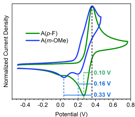
Fig. 1 Cyclic voltammograms of A(m-OMe) , blue line) and A(p-F) , green line) at 298 K at a scan rate of 100 mV s -1 in 0.1 M TBAPF 6 in CH 2 Cl 2 . Potentials have been corrected using ferrocene as reference.
