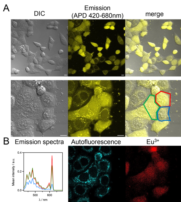
Fig. 9 2P imaging ( \lambda_{\text{ex}} = 720 nm) of living HeLa cells incubated 1 h with mTAT[SucNH-Ar-Ar-L-Eu] (5 \mu M) and dFFLIPTAT (1.5 \mu M) in RPMI medium. (A) Left panel: DIC image; Middle panel: luminescence image recorded with 420–680 nm bp APD detection (arbitrarily coloured in yellow); Right panel: merge. Scale bars correspond to 10 \mu m. (B) Left panel: 2P-excited emission spectra (detected with a PMT array and averaged over the whole cell surface) of the cells outlined in red, blue and green in panel A; Middle and right panels: autofluorescence and \text{Eu}^{3+} emission maps (coloured in cyan and red, respectively) obtained by linear unmixing of a 2P-excited spectral image recorded with the PMT.
