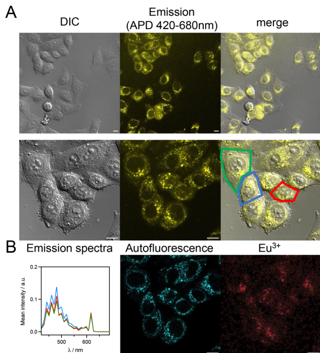
Fig. 6 2PM imaging ( \lambda_{\text{ex}} = 720 nm) of living HeLa cells incubated 1 h with mTAT[SucNH-Ar-Ar-L-Eu] (5 μM) in RPMI medium. (A) Left panel: differential interference contrast (DIC) image; Middle panel: luminescence image recorded with 420–680 nm bp APD detection (arbitrarily coloured in yellow); Right panel: merge. Scale bars correspond to 10 μm. (B) Left panel: 2P-excited emission spectra (detected with a PMT array and averaged over the whole cell surface) of the cells outlined in red, blue and green in panel A; Middle and right panels: autofluorescence and \text{Eu}^{3+} emission maps obtained by linear unmixing of a 2P-excited spectral image recorded with the PMT.
