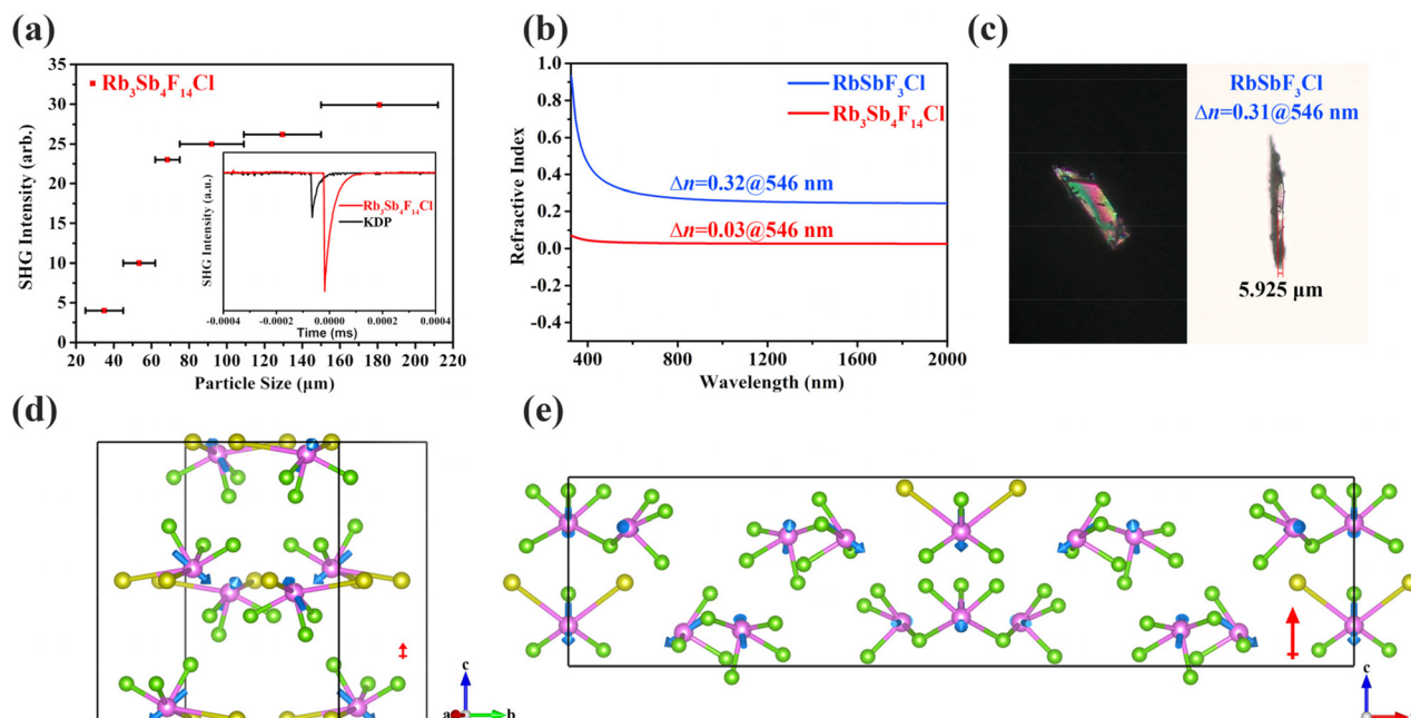
Fig. 3 (a) The phase-matching curve for Rb 3 Sb 4 F 14 Cl. Inset: SHG intensity with KDP as the reference (150–212 μm). (b) Calculated birefringence for RbSbF 3 Cl and Rb 3 Sb 4 F 14 Cl. (c) The experimental birefringence of RbSbF 3 Cl. (d) The orientations of the lone pair of electrons in the unit cell of Rb 3 Sb 4 F 14 Cl. (e) The orientations of the lone pair of electrons on Sb 3+ within a single cell in Rb 3 Sb 4 F 14 Cl. The direction of the overall dipole moments is highlighted by a red arrow.
