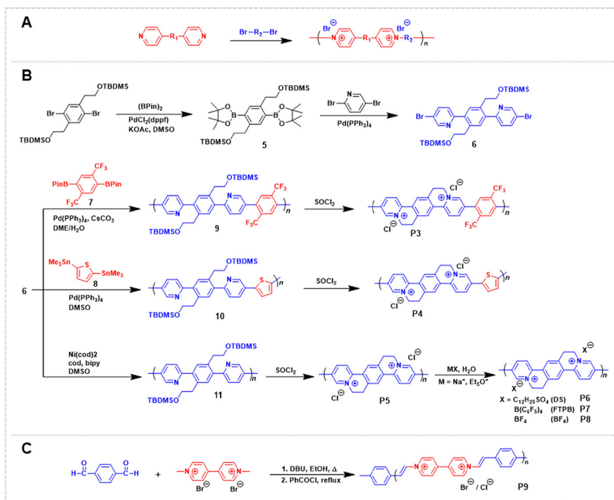
Fig. 2 (A) The common method used for the synthesis of non-conjugated MCPs. (B and C) Synthesis of pyridium-containing CMCPs via (B) nucleophilic substitution reactions and (C) aldol-type polycondensations. Adapted with permission from (B) ref. 48 (Copyright 2009 American Chemical Society), ref. 49 (Copyright 2014 Wiley-VCH GmbH), and (C) ref. 50 (Copyright 1989 Wiley-VCH), respectively.
