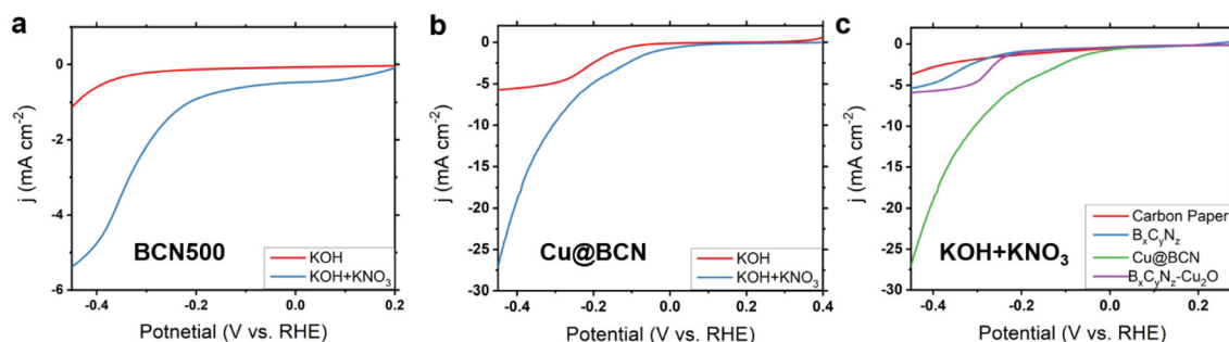
Fig. 7 Voltammetric (LSV) curves of BCN500 (a) and Cu@BCN (b) on carbon paper under alkaline conditions (1 M KOH) with and without the presence of nitrate ions (0.1 M \text{KNO}_3 ). Comparison of the \text{NO}_3\text{RR} activity of the bare carbon paper substrate, BCN500, and Cu@BCN in 1 M KOH + 0.1 \text{KNO}_3 electrolyte (c).
