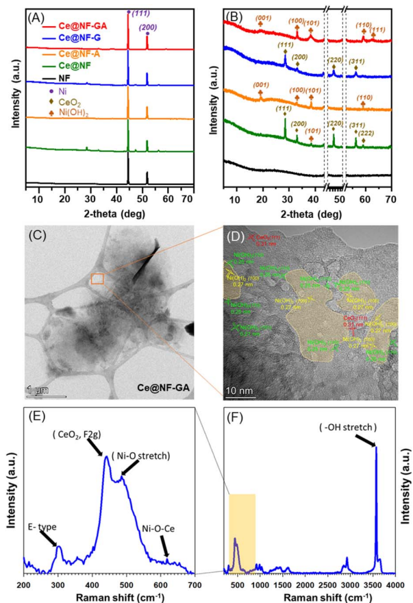
Fig. 2 XRD patterns (A), corresponding magnification of XRD patterns (B) of the as-prepared samples, TEM and HR-TEM image (C and D) and Raman spectra (E and F) of \text{Ce@NF-GA} .
