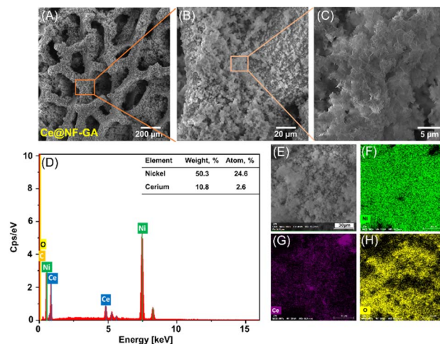
Fig. 1 SEM images (A–C), EDX spectra (D) and elemental mapping (E–H) of the as-prepared \text{Ce@NF-GA} sample.
