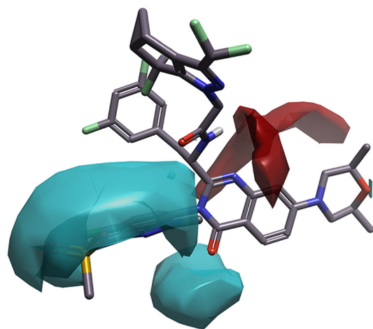
Fig. 8 Activity Atlas™ analysis with GSK878 (12) as a reference. (A) Activity cliff summary showing areas of favoured negative (blue) and positive (red) electrostatics. (B) Activity cliff summary showing areas of favourable (green) and unfavourable (purple) hydrophobics.
