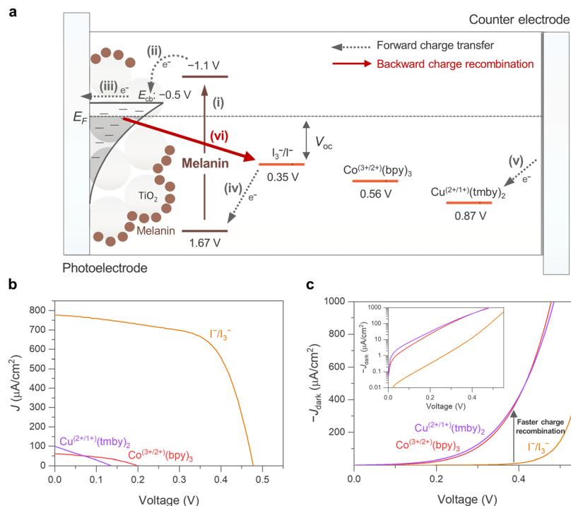
Fig. 2 Operational principle and performance investigation of melanin-DSSCs with varied electrolytes. (a) Energy level diagram showing the quasi-Fermi level ( E_F ) conduction band of the TiO 2 , the HOMO and LUMO levels of melanin based on the calculation result, and the redox potentials of different electrolyte mediators, all referenced versus the normal hydrogen electrode (NHE). This diagram demonstrates the free energy differences driving forward charge transfer (dotted gray arrows) and backward charge recombination (solid red arrow). (b) J-V curves obtained under standard AM 1.5G sunlight at 100 mW cm -2 for melanin-DSSCs with different redox mediators, employing a mask to prevent the problem of overestimation. (c) Dark current curves of the melanin-DSSCs with different redox mediators, revealing highly accelerated charge recombination behavior at high-voltage bias in melanin-DSSCs with the metal-complex based mediators ( \text{Co}^{(3+/2+)}(\text{bpy})_3 and \text{Cu}^{(2+/1+)}(\text{tmby})_2 ). The inset shows the same graph with a logarithmic scale, indicating the overall charge recombination characteristics.
