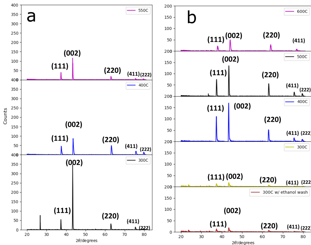
Fig. 1 XRD patterns of initial molten salt synthesis products (a) NiO(100) nanocubes and (b) \text{Li}_2\text{O} -reduced nanoparticles.
