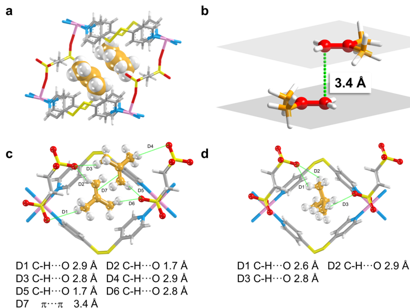
Fig. 3 (a) 2 iso- \text{C}_4\text{H}_8 molecules adsorbed in one pore cage of ZU-603 as revealed by single crystal analysis; (b) the packing diagram of 2 iso- \text{C}_4\text{H}_8 molecules adsorbed within one pore cage of ZU-603 as revealed by single crystal analysis; (c) the specific binding sites of iso- \text{C}_4\text{H}_8 on ZU-603 as revealed by single crystal experiments; (d) the specific binding sites of iso- \text{C}_4\text{H}_{10} on ZU-603 as revealed by DFT-D calculations (color code: silver, C; white, H; red, O; blue, N; yellow, S; pink, Cu; orange, C of the adsorbed molecules).
