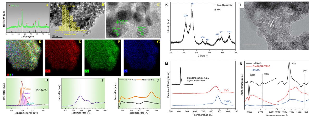
Fig. 7 Morphology, structure and property of the \text{ZnCrO}_x and \text{ZnAlO}_x spinels. (A) XRD pattern, (B) TEM image, (C) HR-TEM image, (D)–(G) STEM-EDX elemental mapping, (H) O 1s XPS spectra, (I) \text{H}_2 -TPR profile, and (J) \text{CO}_2 -TPD profile of the \text{ZnCrO}_x oxide. Reprinted with permission from Guo et al. Copyright (2024), American Chemical Society. 43 (K) XRD pattern, (L) HR-TEM image with a scale bar of 10 nm, (M) \text{H}_2 -TPR profiles normalized by weight and the relative intensity of the standard sample \text{Ag}_2\text{O} was divided by 50, (N) FTIR subtraction spectra relative to adsorption of DTBPy of the \text{ZnAlO}_x oxide. Reprinted with permission from Ni et al. Copyright (2018), The Authors. 41
