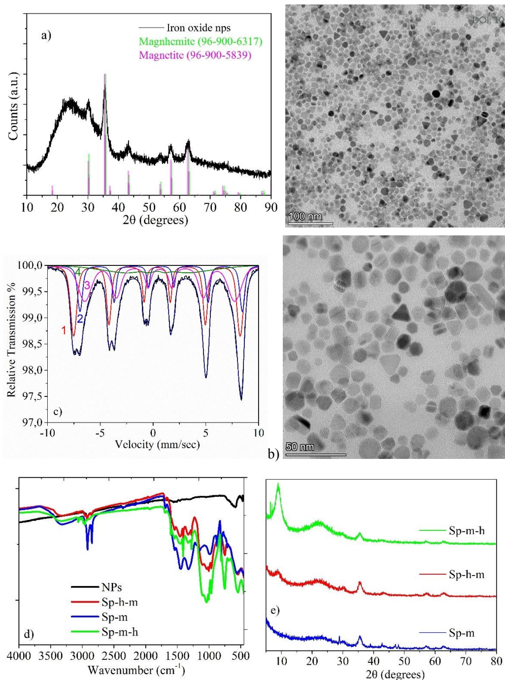
Figure 1. a) The XRD pattern, b) TEM images, and c) the Mössbauer spectrum of the iron oxide NPs (non-stoichiometric magnetite), d) the FT-IR spectra of all the evaluated materials (non-stoichiometric magnetite NPs and the modified sponges), and e) the XRD patterns of the three modified sponges.
