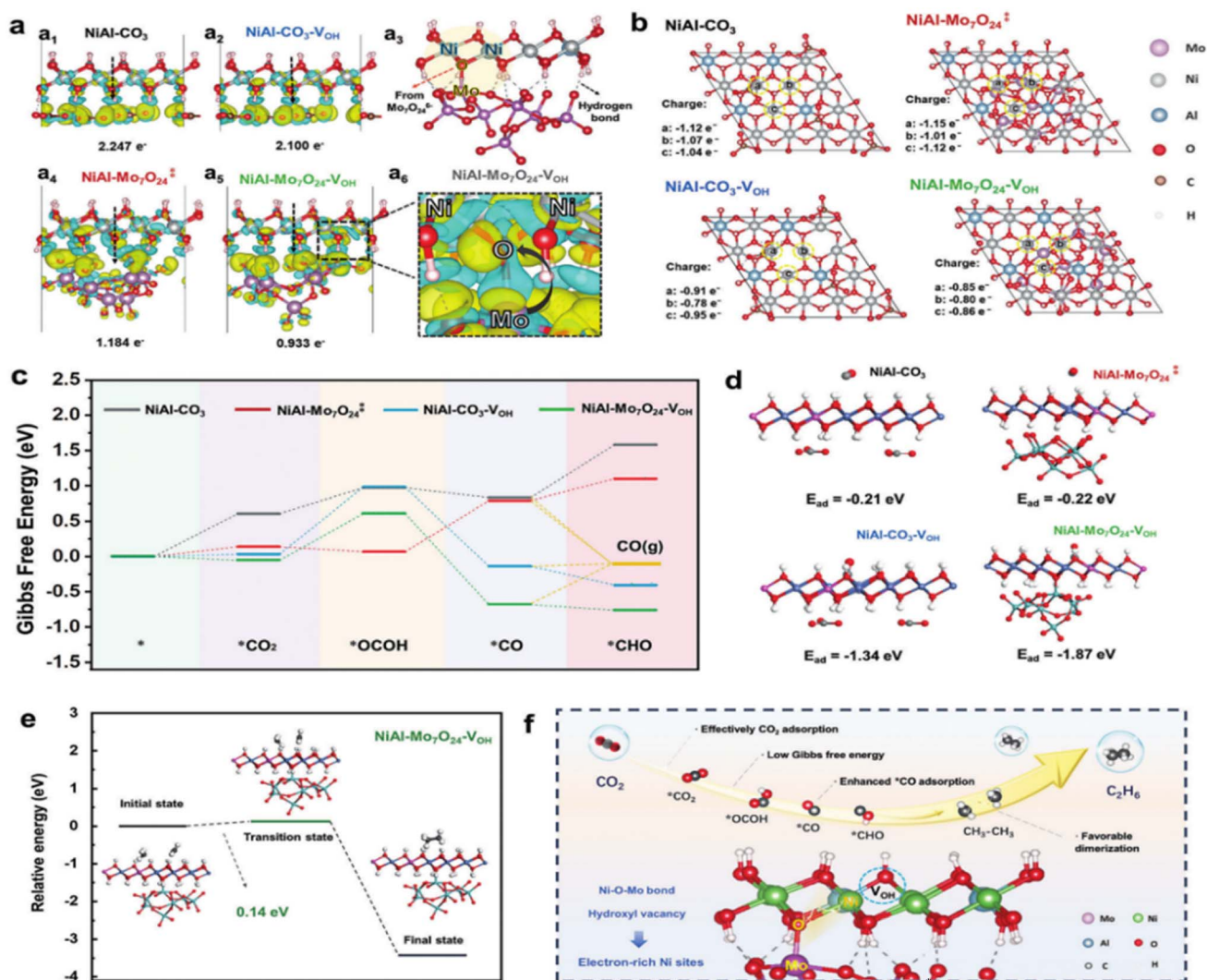
Fig. 10 (a) Differential charge density calculations for (a 1 ) NiAl-CO 3 , (a 2 ) NiAl-CO 3 -V OH , (a 4 ) NiAl-Mo 7 O 24 2- , (a 5 ) NiAl-Mo 7 O 24 -V OH and (a 6 ) locally amplified spectra of NiAl-Mo 7 O 24 -V OH ; blue regions represent charge loss and yellow regions represent charge accumulation. (a 3 )
