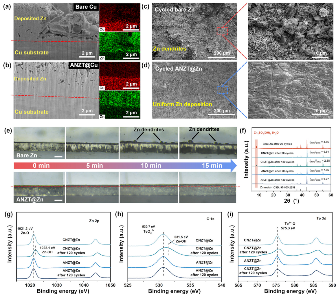
Fig. 4 Side-view SEM images of FIB-milled (a) bare Cu and (b) ANZT@Cu electrodes with 2.5 mA h cm -2 Zn metal deposition (at 5 mA cm -2 ) and the corresponding EDS mapping results. SEM images of (c) bare Zn and (d) ANZT@Zn electrodes after 50 cycles at 5 mA h cm -2 /2.5 mA h cm -2 , and the enlarged SEM images are inserted on the right. (e) In situ optical microscopy measurement records the Zn deposition morphology on bare Zn and ANZT@Zn anodes (100 μm Zn foil) at a current density of 30 mA cm -2 , scale bar: 100 μm. (f) XRD patterns of bare Zn, CNZT@Zn, and ANZT@Zn anodes after different cycle numbers (in symmetric cells at 1 mA cm -2 /1 mA h cm -2 ), with calculated I_{(002)}/I_{(101)} values. High resolution XPS spectra of (g) Zn 2p, (h) O 1s, and (i) Te 3d of CNZT and ANZT interlayers after 120 cycles (in symmetric cells at 1 mA cm -2 /1 mA h cm -2 ).
