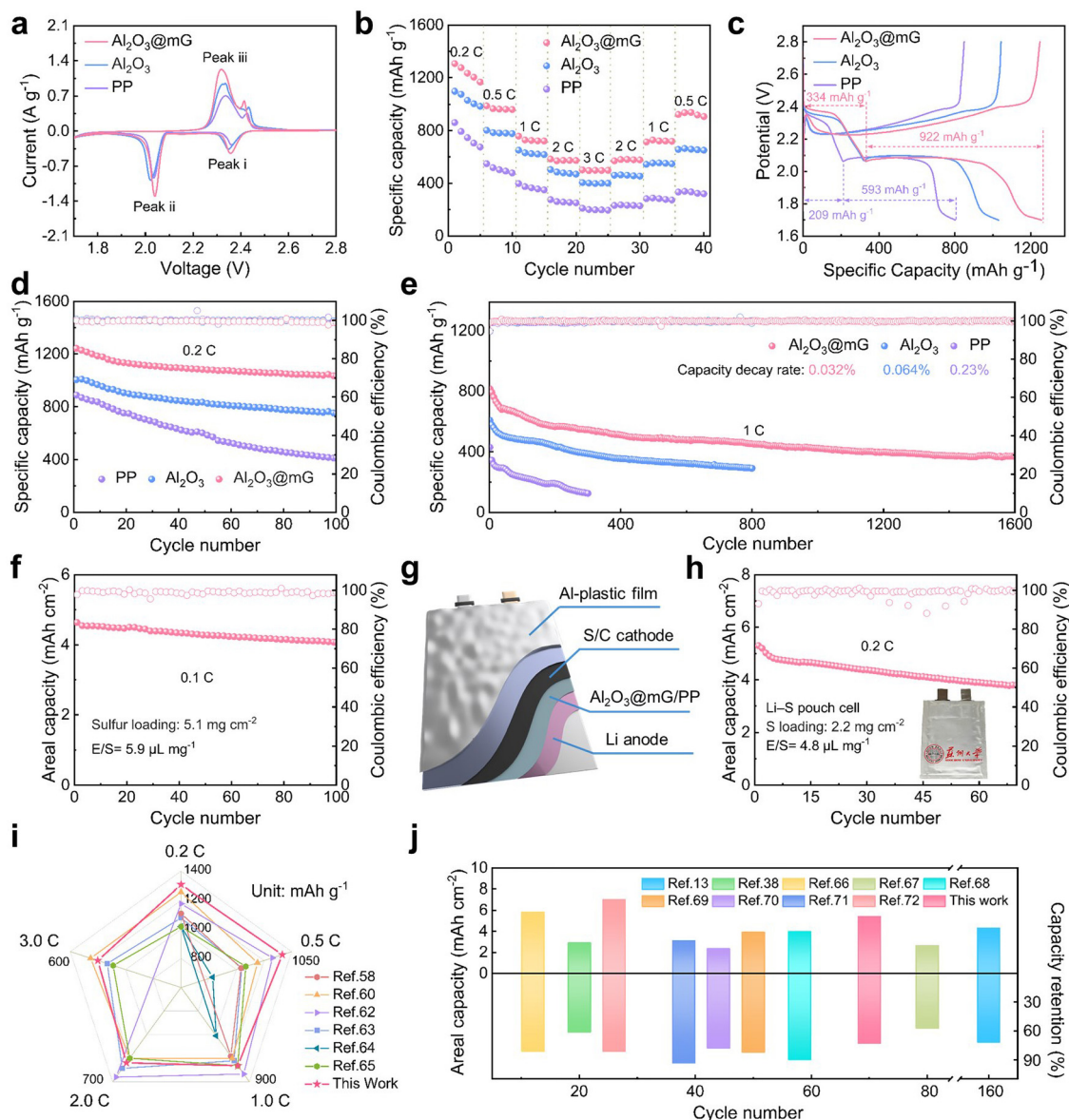
Fig. 6 Electrochemical performance. (a) CV profiles of Li-S batteries with \text{Al}_2\text{O}_3@\text{mG}/\text{PP} , \text{Al}_2\text{O}_3/\text{PP} , and PP separators at 0.05 \text{ mV s}^{-1} . (b) Rate performances. (c) GCD profiles at 0.2 \text{ C} . (d) and (e) Cycling performances at 0.2 \text{ C} and 1.0 \text{ C} , respectively. (f) Cyclic performances of Li-S batteries equipped with \text{Al}_2\text{O}_3@\text{mG} modified separators with a sulfur loading of 5.1 \text{ mg cm}^{-2} . (g) Schematic of the pouch cell equipped with the \text{Al}_2\text{O}_3@\text{mG} modified separator. (h) Cycling performance of an assembled pouch cell at 0.2 \text{ C} . Comparison of (i) the coin cell and (j) the pouch cell between this work and related counterparts in Li-S batteries.
