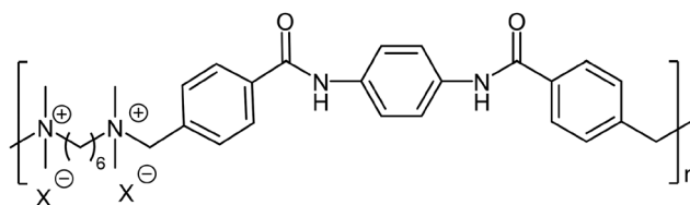
Fig. 1 Structure of poly[(dimethylimino) hexane-1,6 diyl(dimethylimino)methylene-1,4-phenylenecarbonylimino-1,4-phenylene-iminocarbonyl-1,4-phenylenemethylene dihalide], X = Cl - or F - as counterions. Ionene solutions/gels based on this structure are denoted from now on as 6-Cl or 6-F ionenes, where 6 represents the number of methylene groups (CH 2 ) between the two charged quaternary ammonium centres inside the aliphatic chain of each monomer.
