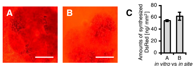
Fig. 4. Fluorescence images and quantitative analysis of DsRed protein synthesized using a cell-free system from (A) immobilized circular DNA ( in situ ) and (B) free circular DNA in solution ( in vitro ). The comparable fluorescence intensities observed in (A) and (B) indicate that immobilization did not impede protein synthesis. (C) Quantitative comparison of DsRed yields from (A) immobilized circular DNA and (B) free circular DNA. Fluorescence intensity was quantified using ImageJ software. Error bars represent the standard deviation of three independent experiments ( n = 3 ). Scale bar = 1 mm.
