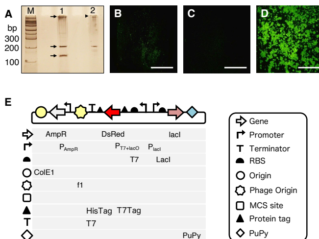
Fig. 1. (A) Electrophoretic mobility shift assay confirming triple-helix formation. A biotinylated homopyrimidine single-stranded oligonucleotide (third strand) was hybridized to the PuPy sequence in pUC19-PyPu to form a triple-helix structure. Arrows indicate DNA fragments of approximately 135, 200, and 5000 bp. The arrowhead indicates the upward-shifted band, which is formed by approximately 135-bp DNA fragment forming a triple helix with a biotinylated oligonucleotide and then binding to streptavidin. The samples were separated on a 12% native PAGE gel and stained using an EzStain Silver Kit. Fluorescence images of DNA immobilized on streptavidin–biotin-modified substrates under three experimental conditions: (B) unlabelled circular DNA (pET21a-PyPu-DsRed), (C) biotinylated single-stranded oligonucleotides functioning as a third strand, and (D) biotinylated circular DNA containing a triple-stranded DNA region. Following immobilization, the substrates were stained with SYBR Green I and visualized using fluorescence microscopy. The enhanced fluorescence intensity observed in (D) confirms the successful formation of the triple-helix structure. Scale bar = 1 mm. (E) plasmid maps of pET21a-PyPu-DsRed.
