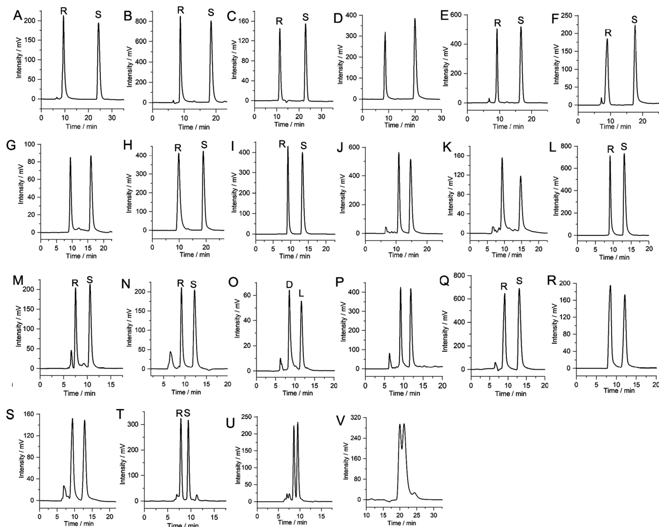
Fig. 4 HPLC chromatograms obtained on CSP-A-packed column A. (A) 4,4'-Difluorobenzoin, (B) 4,4'-dimethylbenzoin, (C) methyl mandelate, (D) 4-chlorobenzhydryl, (E) 4-methylbenzhydryl, (F) 1,1'-bi-2-naphthol, (G) 3-hydroxy-2-butanone, (H) ethyl mandelate, (I) 1-phenylethanol, (J) 1-indanol, (K) ketoprofen, (L) 2-methoxy-2-phenylethanol, (M) 1-phenyl-1-pentanol, (N) benzoin, (O) mandelic acid, (P) 2-phenylcyclohexanone, (Q) 1-(4-fluorophenyl)ethanol, (R) 1-phenyl-1-propanol, (S) 2-phenyl-1-propanol, (T) 1-(4-fluorophenyl)ethanamine, (U) styrene oxide, and (V) amlodipine.
