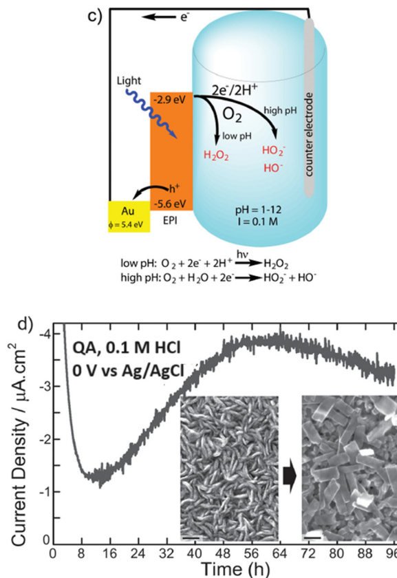
Fig. 12 (a) and (b) Epindolidione (EPI) and QA photocathodes for photoelectrochemical synthesis of H 2 O 2 upon reduction of oxygen. Panel (c) represents the operating mechanism and the energy levels involved. Panel (d) shows the morphological evolution of QA films along the photoelectrocatalysis by scanning electron microscopy. Reproduced from ref. 39 with permission from Wiley Inc., copyright 2016.
