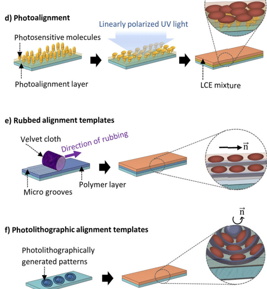
Fig. 7 LCE alignment methods: (1) bulk alignment: (a) electric field: the director aligns with the electric field direction. (b) Magnetic field: mesogens align with the magnetic induction intensity direction. (c) Mechanical stresses: alignment direction follows the stretching direction. (2) Photoalignment: the director can be perpendicular or parallel to the light vector's direction. (2) Interfacial alignment: (e) rubbed alignment templates: the direction of mechanical friction during rubbing defines the alignment direction of the mesogens. (f) Photolithographic alignment templates: microchannel direction dictates the alignment of mesogens within the LCE.
