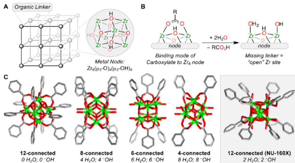
Fig. 2 (A) Simplified representation of a metal-organic framework (MOF) showing metal ions or cluster nodes and ditopic organic linkers. The structure of the Zr_6 node in all Zr-MOFs, Zr_6(\mu_3-O)_4(\mu_3-OH)_4 , is shown here. (B) Depiction of one carboxylate ligand binding to the Zr_6 node, highlighting the bridging Zr-O-Zr motif. Missing carboxylate linkers, such as in missing-linker defect sites or nodes with lower connectivity, are typically replaced by one terminal aqua and one terminal hydroxo ligand. (C) Representation of the ideal node structure in 12-, 8-, 6-, and 4-connected nodes in Zr-MOFs (with the exception of NU-160X ( X = 0, 1, 2 ), in which the 12-connected Zr_6 node adopts the rare hexagonal prismatic geometry). The numbers of terminal H_2O and -OH ligands coordinated to the ideal node are listed below each node diagram. Reproduced from ref. 37 with permission from American Chemical Society, Copyright 2019.
