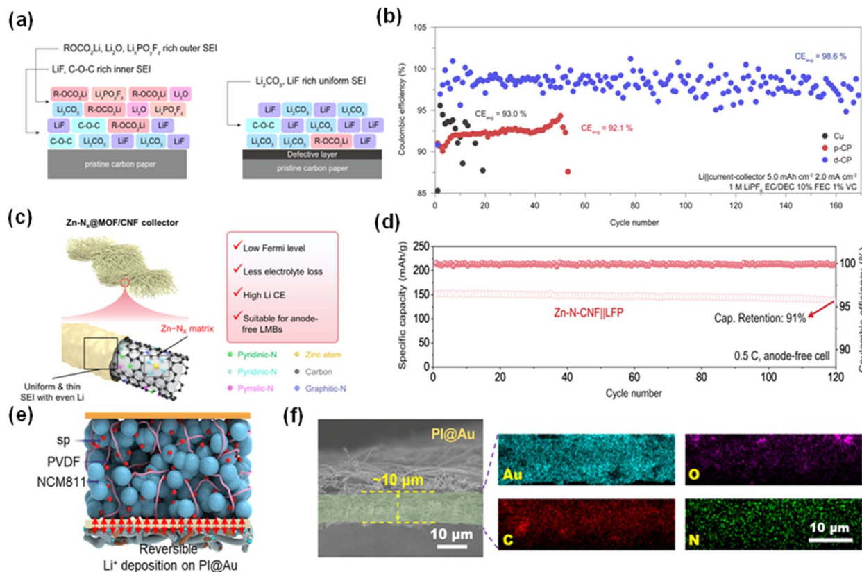
Fig. 13 New types of current collector and their performance. (a) The proposed SEI chemical composition on the p-CP CC and d-CP CC. (b) Li plating efficiency on bare Cu, p-CP and d-CP at 2 mA cm -2 . 91 Reproduced with permission. Copyright 2021, Springer Nature. (c) Advantages of the Zn-N-CNF CC over traditional CCs. (d) Cycling performance of a Zn-N-CNF||LFP full-cell over 120 cycles. 70 Reproduced with permission. Copyright 2024, Elsevier. (e) Reversible Li ion deposition on PI@Au. (f) Energy dispersive spectroscopy (EDS) images of PI@Au. 93 Reproduced with permission. Copyright 2023, Elsevier.
