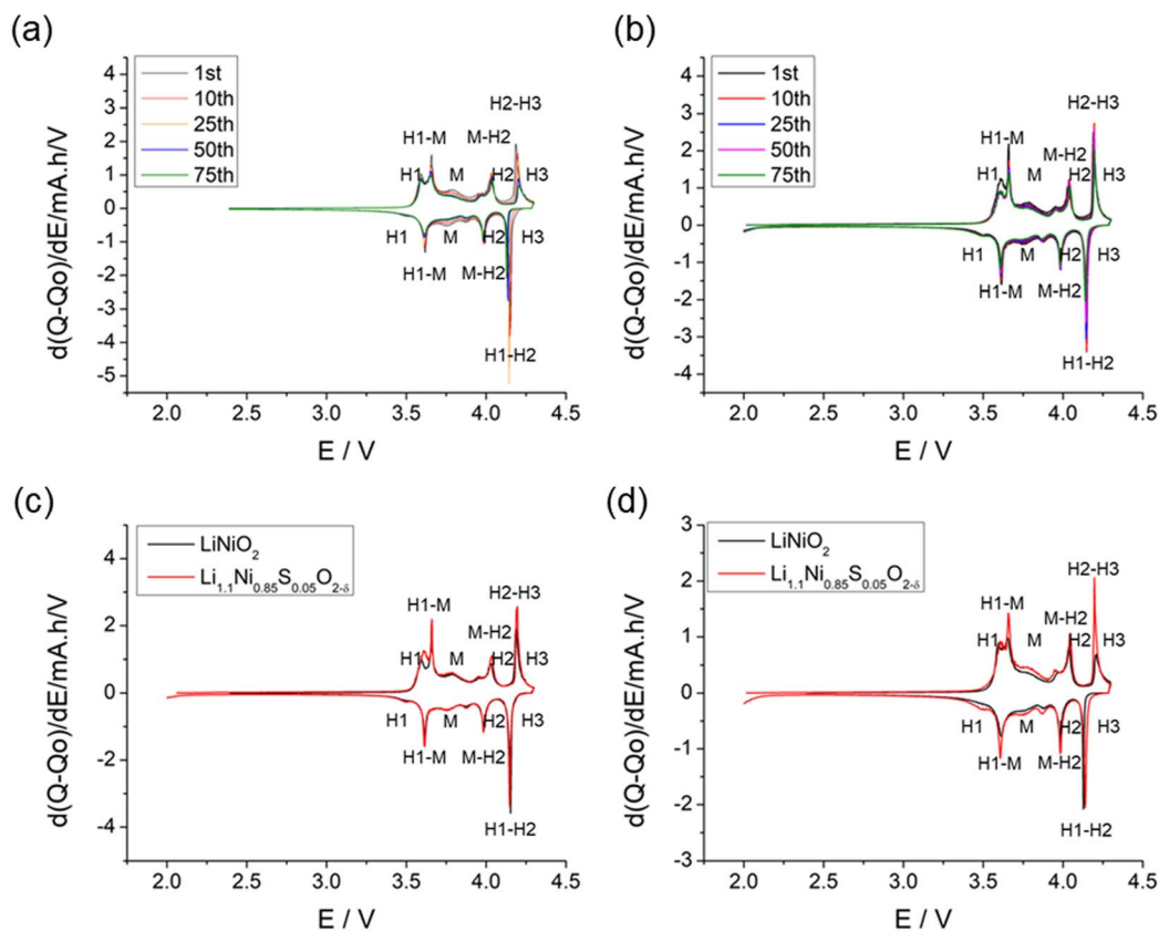
Fig. 10 dQ/dV curves of (a) LiNiO_2 and (b) Li_{1.1}Ni_{0.85}S_{0.05}O_{2-x} prepared through co-precipitation route; (c) comparison of LiNiO_2 and Li_{1.1}Ni_{0.85}S_{0.05}O_{2-x} at 1st cycle. (d) Comparison of LiNiO_2 and Li_{1.1}Ni_{0.85}S_{0.05}O_{2-x} at 75th cycle showing the clear preservation of H2-H3 transition in the latter.
