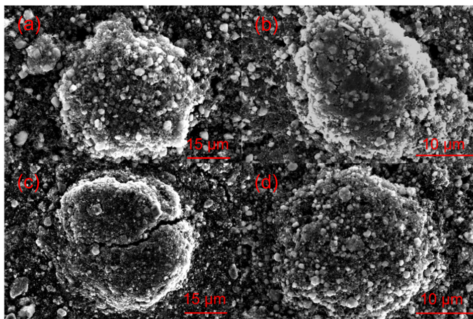
Fig. 11 SEM images of (a) pristine LiNiO_2 ; (b) pristine Li_{1.1}Ni_{0.85}S_{0.05}O_{2-x} (c) LiNiO_2 after 200 cycles. (d) Li_{1.1}Ni_{0.85}S_{0.05}O_{2-x} after 200 cycles.
