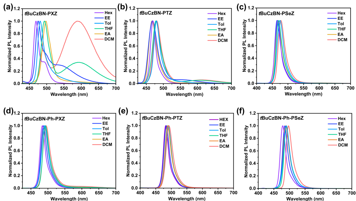
Fig. 3 Solvatochromic effect on PL spectra in 10^{-5} M solution. (a) tBuCzBN-PXZ , (b) tBuCzBN-PTZ , (c) tBuCzBN-PSeZ , (d) tBuCzBN-Ph-PXZ , (e) tBuCzBN-Ph-PTZ and (f) tBuCzBN-Ph-PSeZ . Hex: n -hexane; EE: diethyl ether; Tol: toluene; THF: tetrahydrofuran; EA: ethyl acetate; DCM: dichloromethane.
