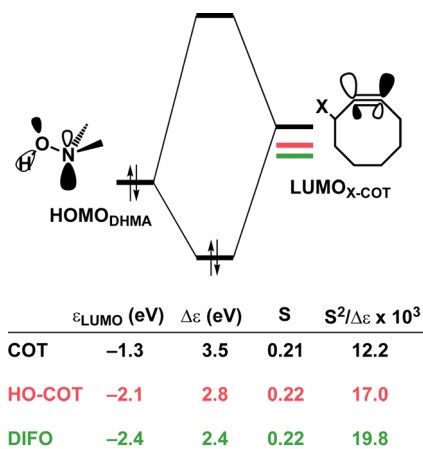
Fig. 5 Schematic diagrams with LUMO energies, energy gaps \Delta\varepsilon , overlaps S, and values of 10^3 \times S^2/\Delta\varepsilon term associated with the key donor–acceptor interaction between HOMO DMHA –LUMO X-COT along with the retro-Cope elimination reactions between COT, HO-COT, and DIFO with DMHA. All were computed at the consistent geometries where the length of the C \cdots H bond is 1.60 Å at ZORA-BP86/TZ2P.
