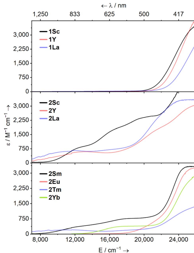
Fig. 2 Solution UV-Vis-NIR spectra of [M(NHAr iPr ) 6 ](II) (1M, M = Sc, Y, La; top) and [M(NHAr iPr ) 6 ] (2M, middle, M = Sc, Y, La; bottom, M = Sm, Eu, Tm, Yb) – as 1 mM solutions in Et 2 O between 7000–26 000 cm -1 (1429–385 nm) at ambient temperature.
