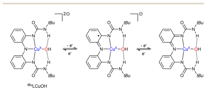
Scheme 9 Characterized oxidation states reached via reduction/oxidation of ^{tBu}LCuOH . Adapted from ref. 73.
