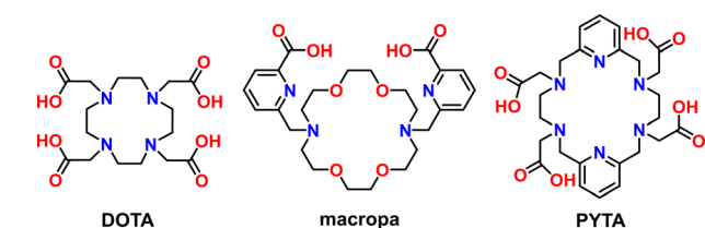
Scheme 1 Chemical structures of the chelators used in this work.
